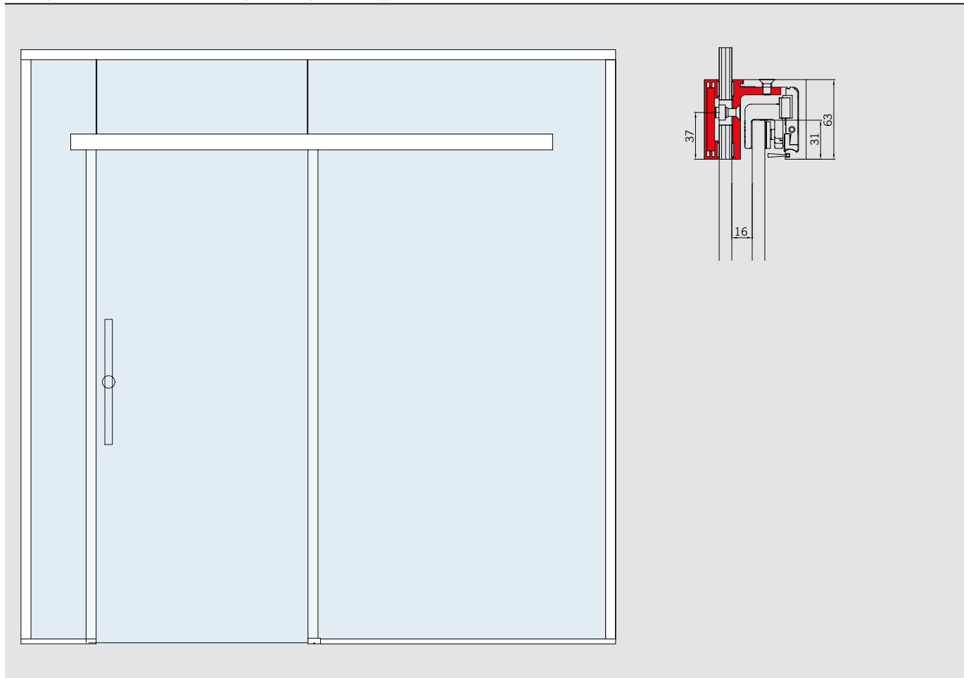
Example view for AGILE 150 with glass overpanel and glass side elements
