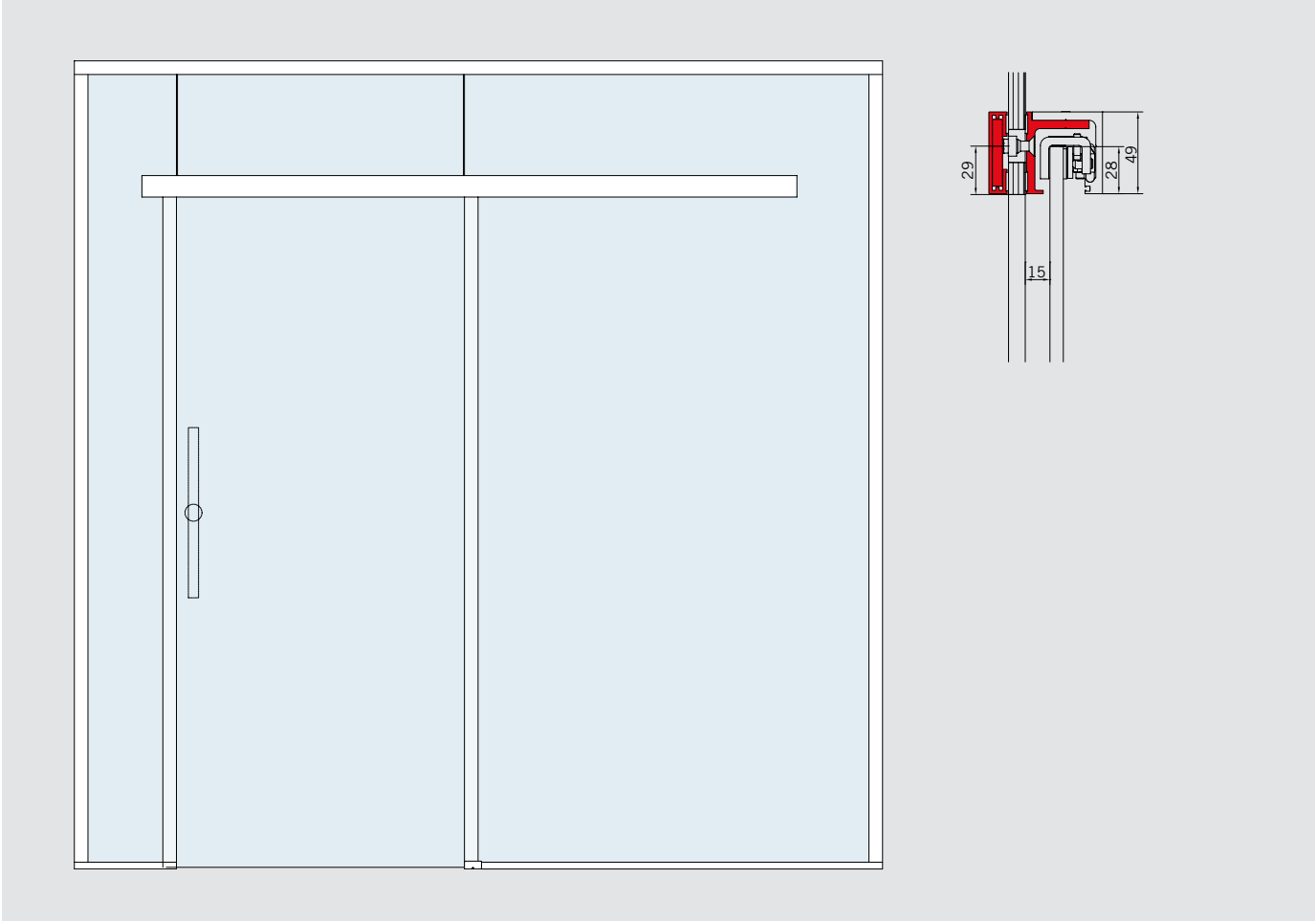
Example view for AGILE 50 with glass overpanel and glass side elements
