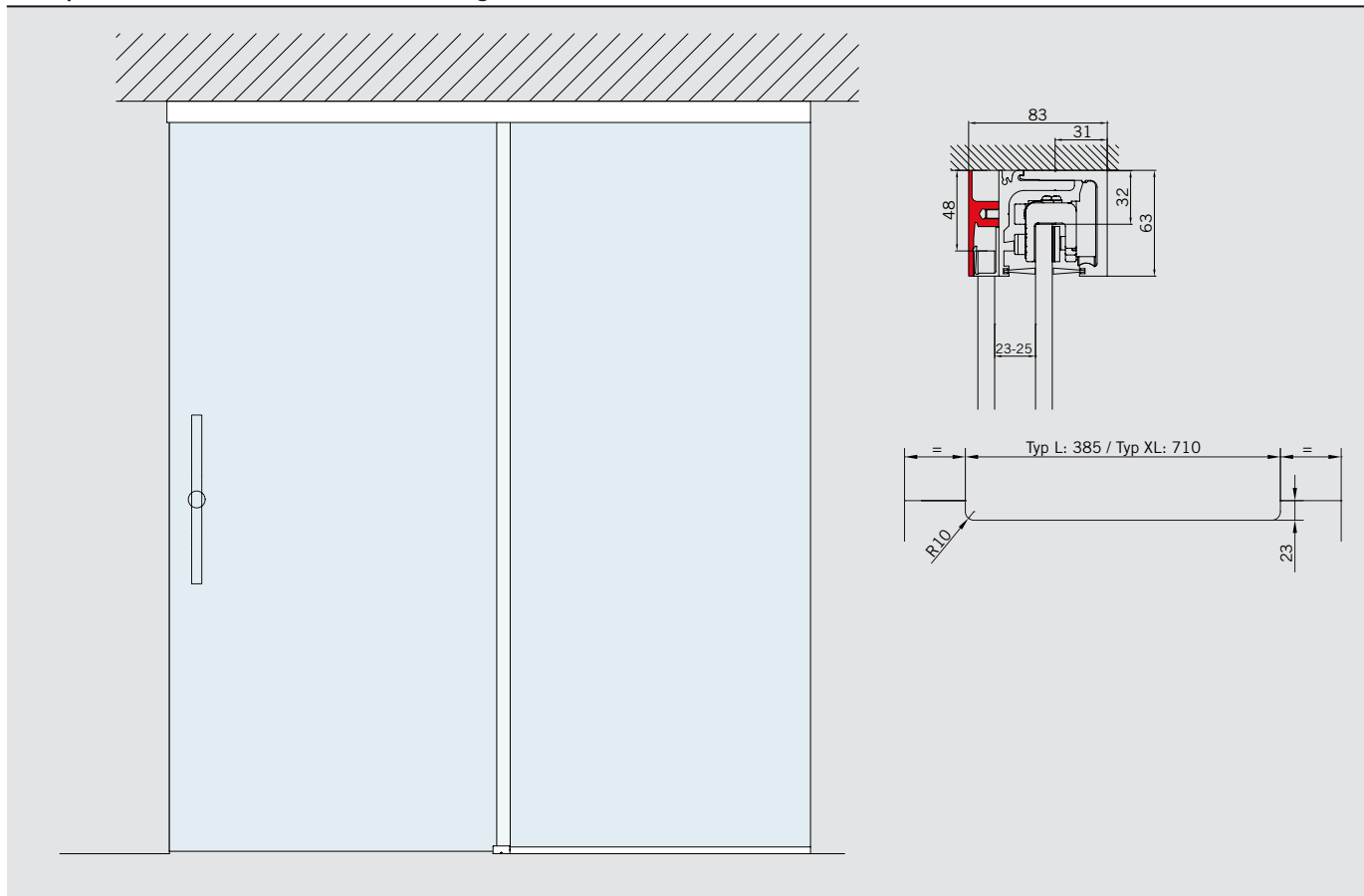
Example view for AGILE 150 DORMOTION with glass overpanel and glass side elements
