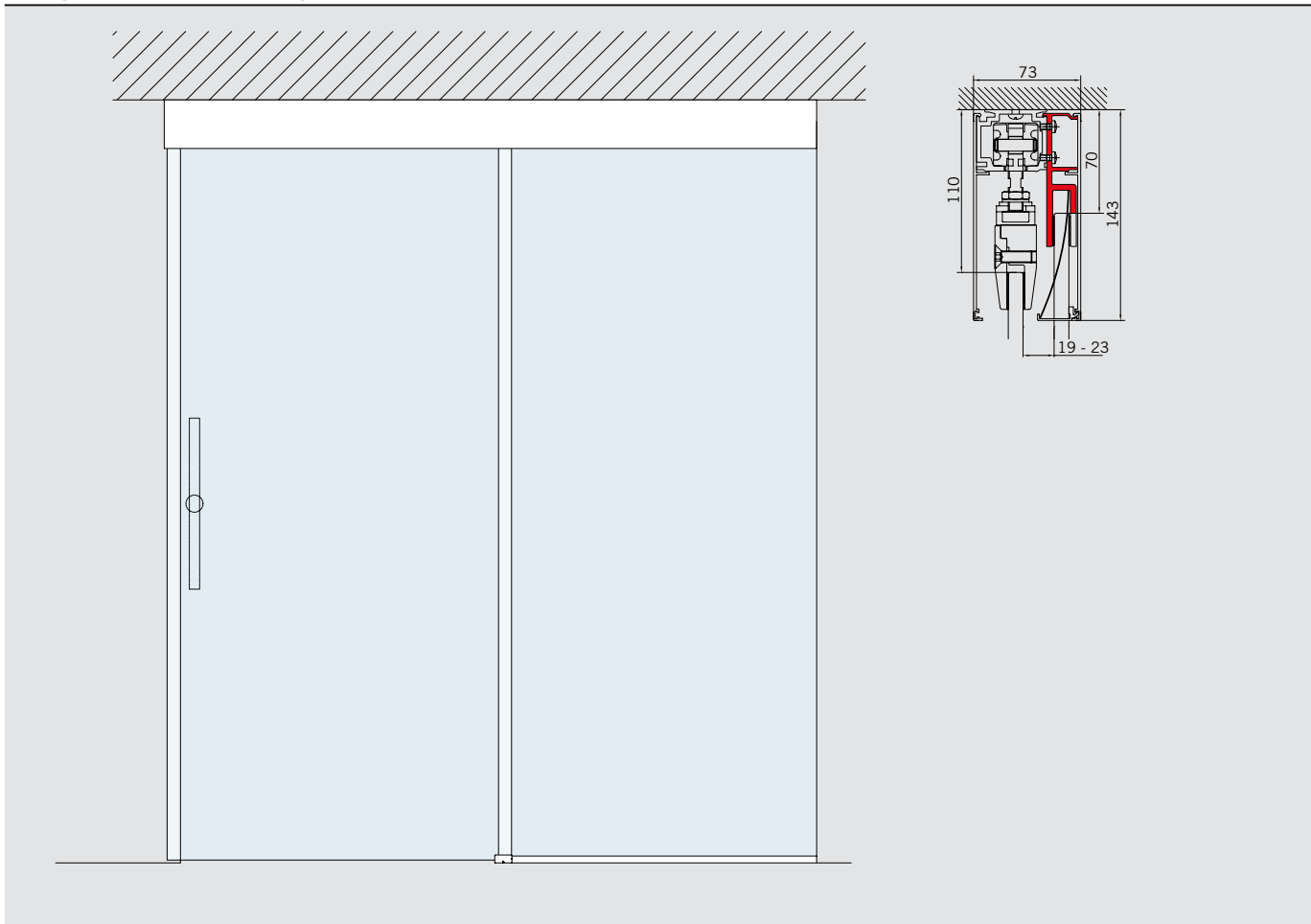
Example view for RS 120 with glass side elements
