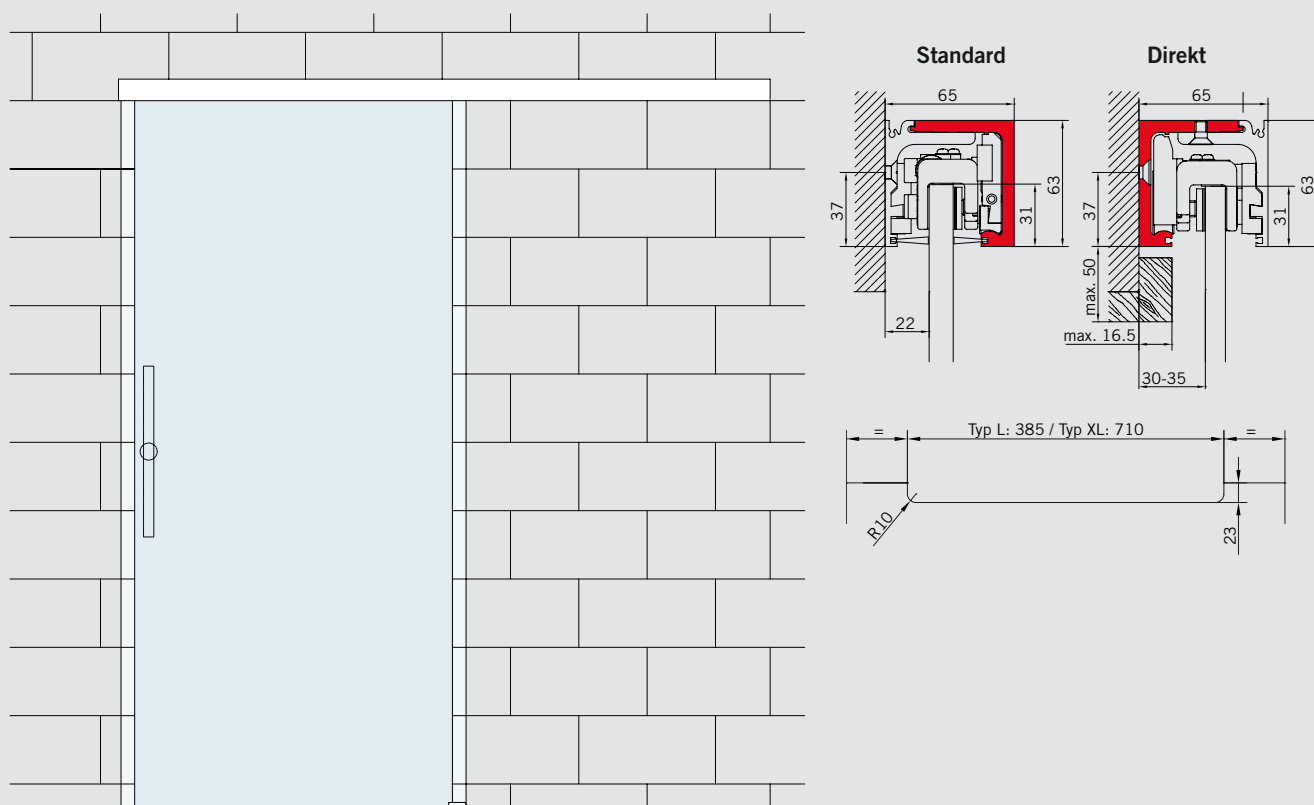
Example view for AGILE 150 DORMOTION installation at wall, standard / direct fixing at track/wall
