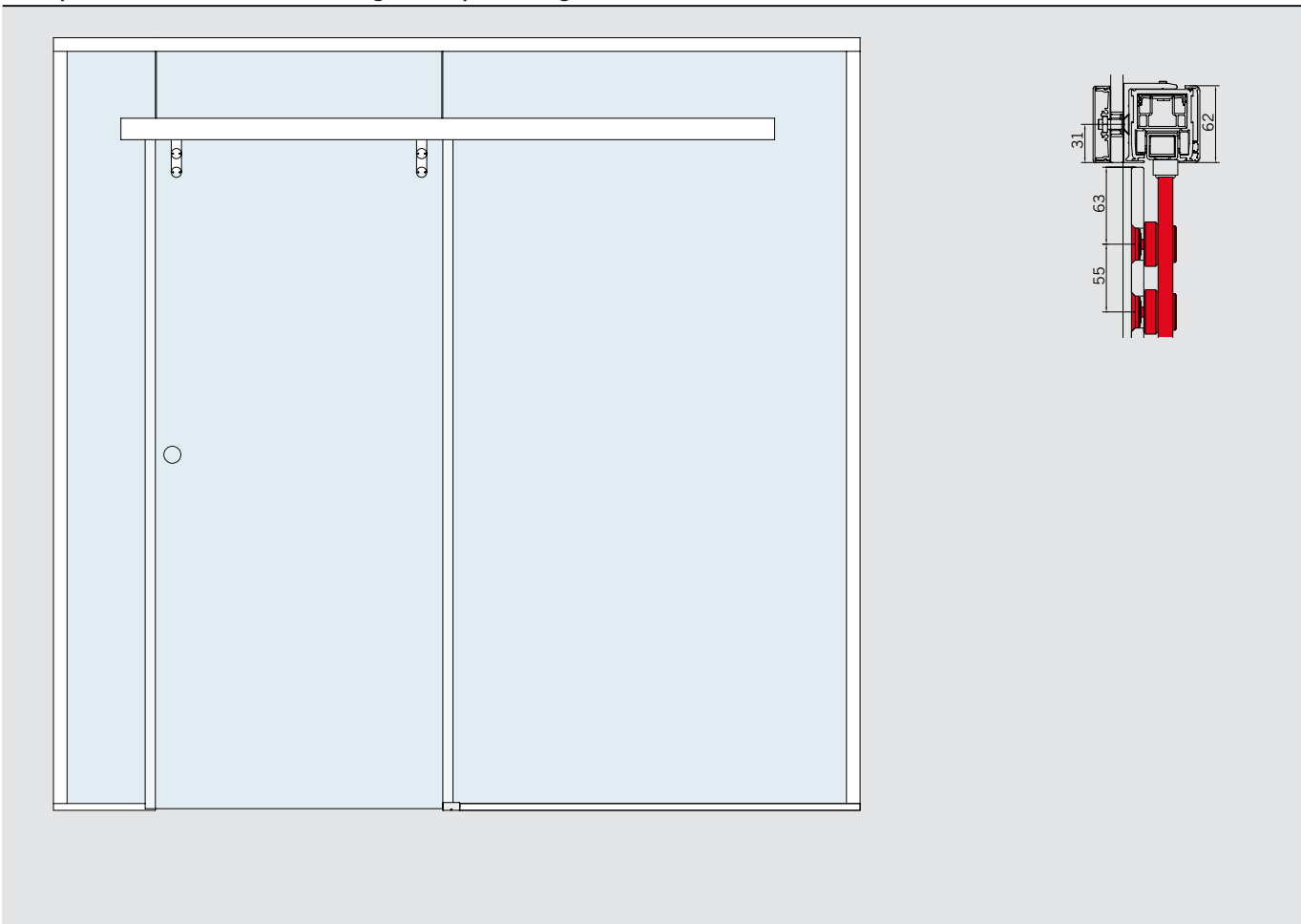
Example view for CS 80 MAGNEO with glass overpanel and glass side elements
