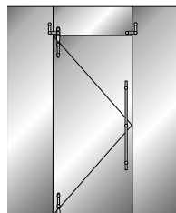
Door type 15 + 1 Overpanel/side element connector
