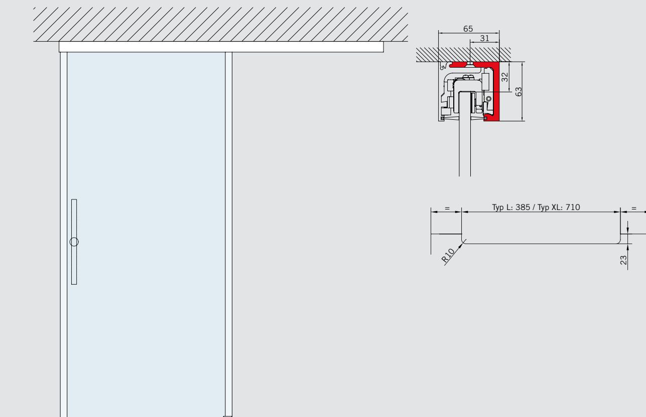
Example view for AGILE 150 DORMOTION installation at ceiling
