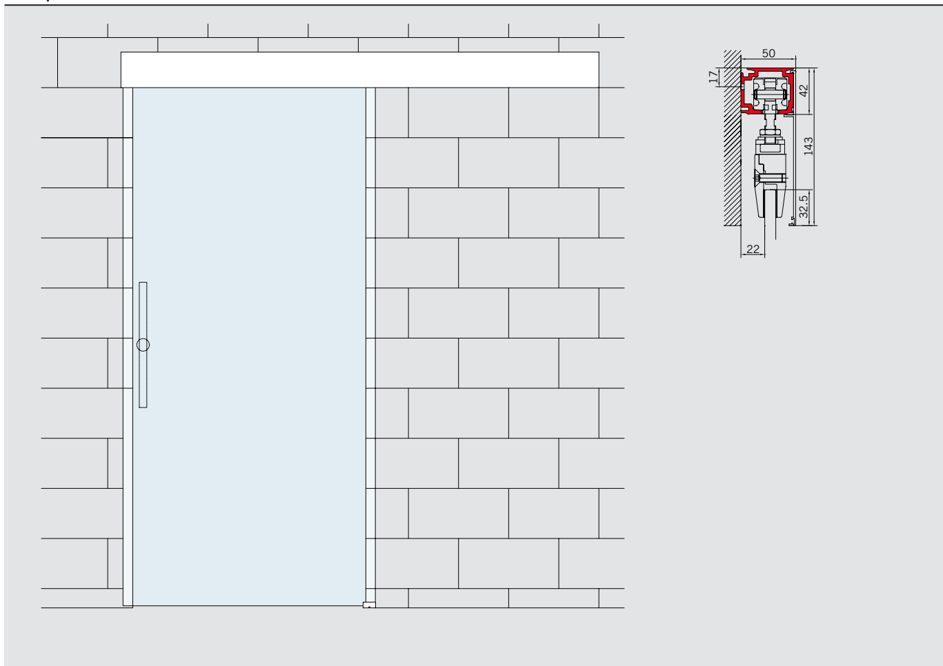
Example view for RS 120 installation at wall
