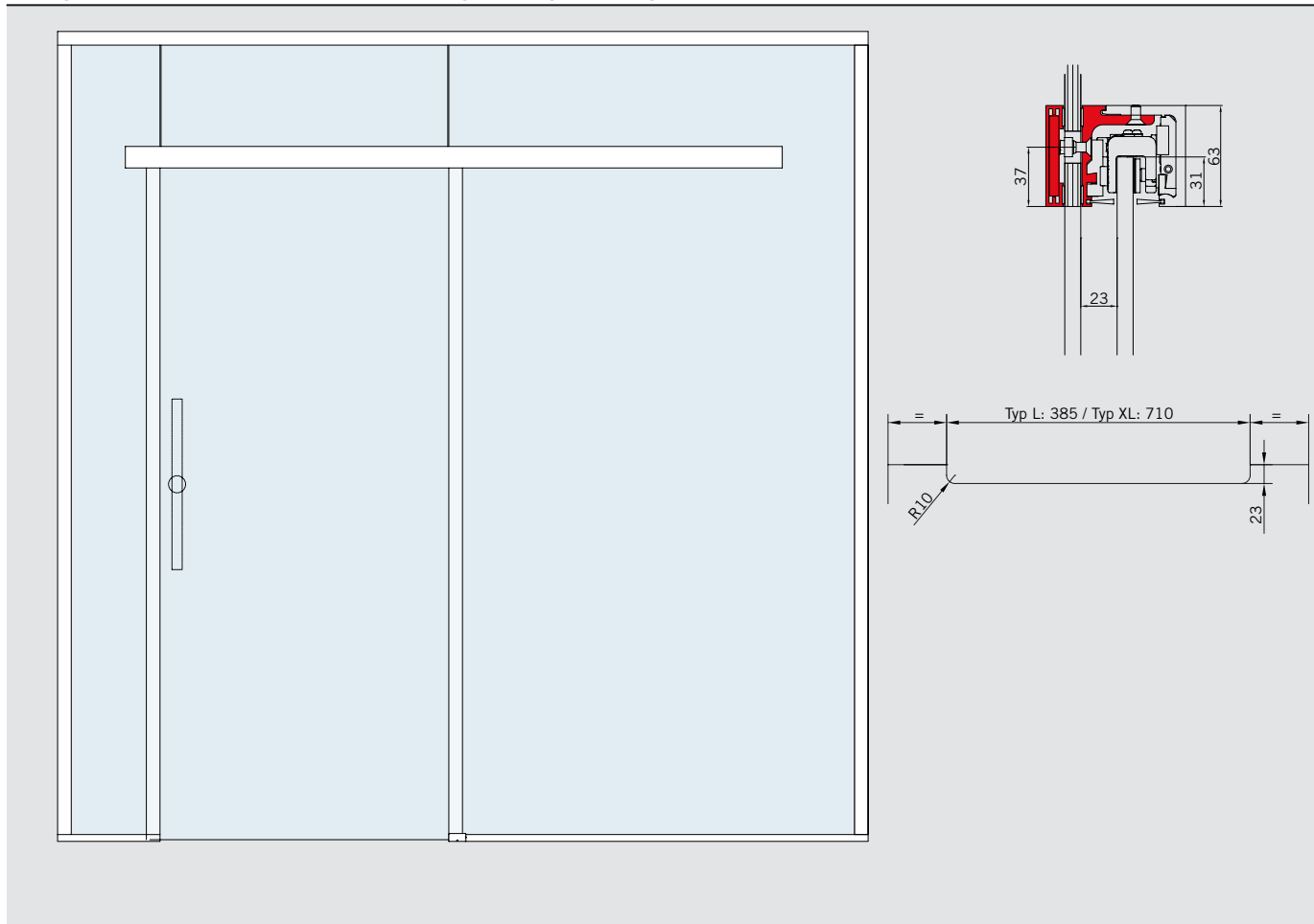
Example view for AGILE 150 DORMOTION with glass overpanel and glass side elements
