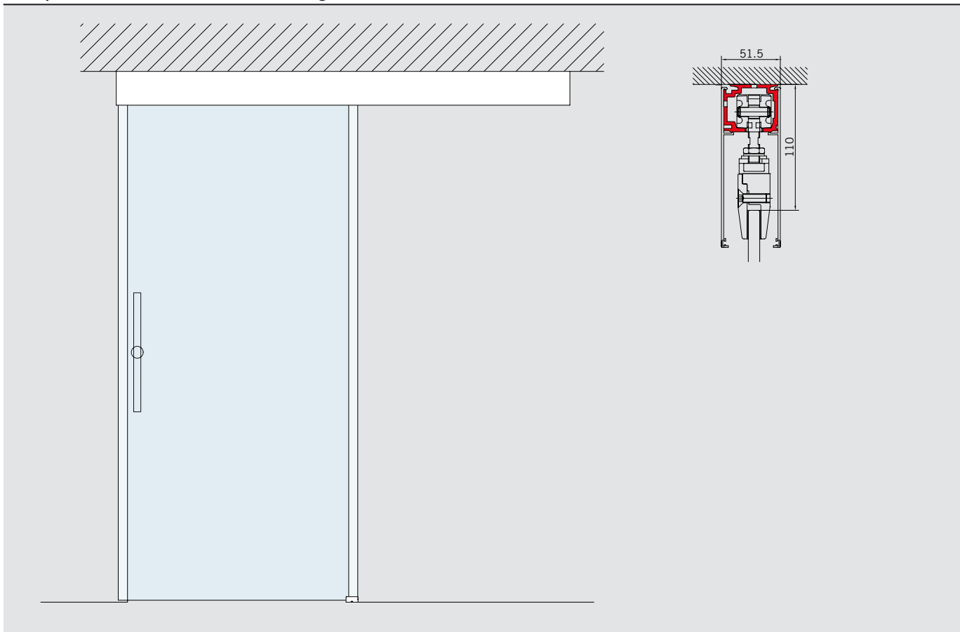
Example view for RS 120 with glass side elements
