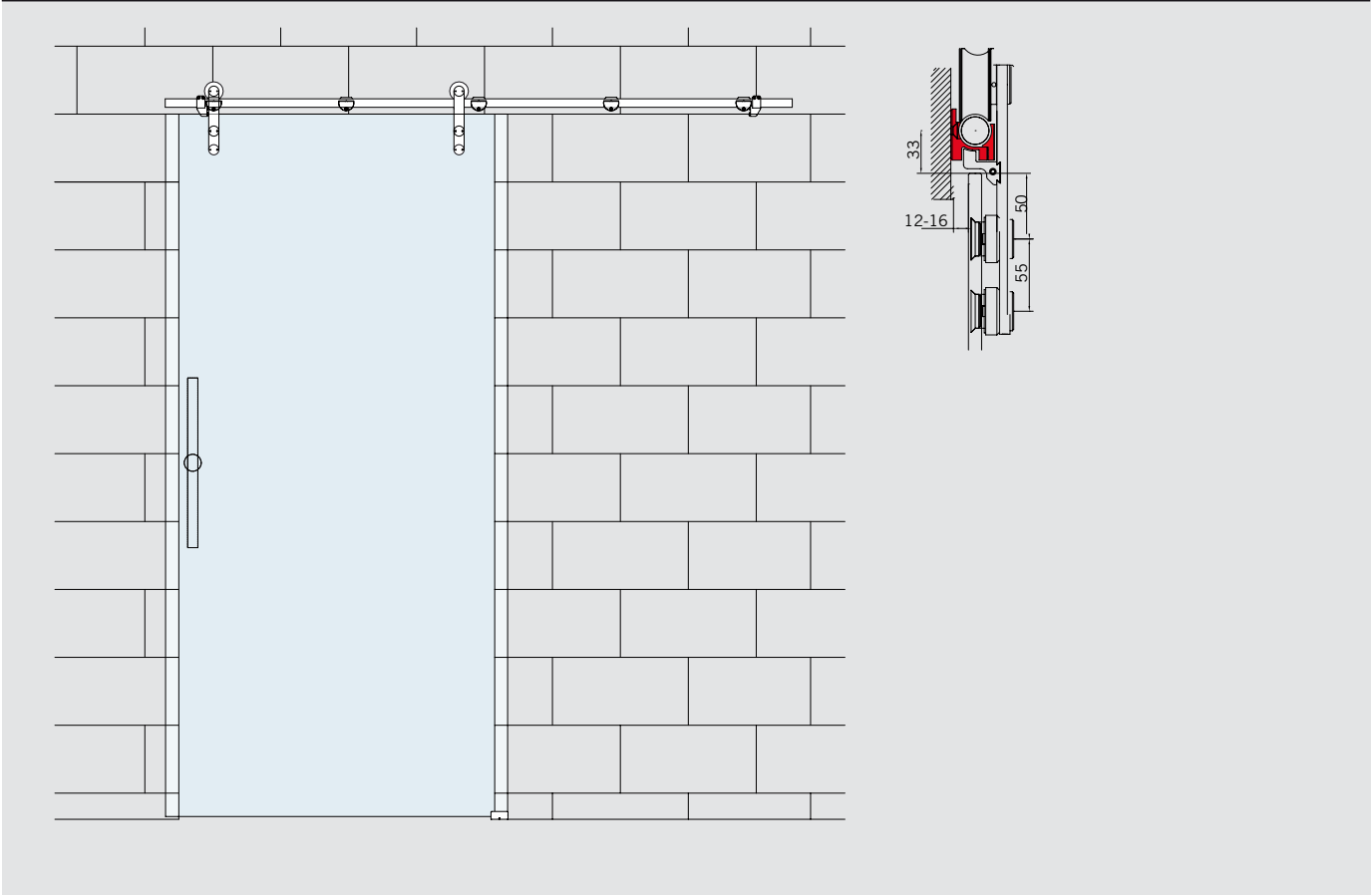
Example view for MANET installation at wall
